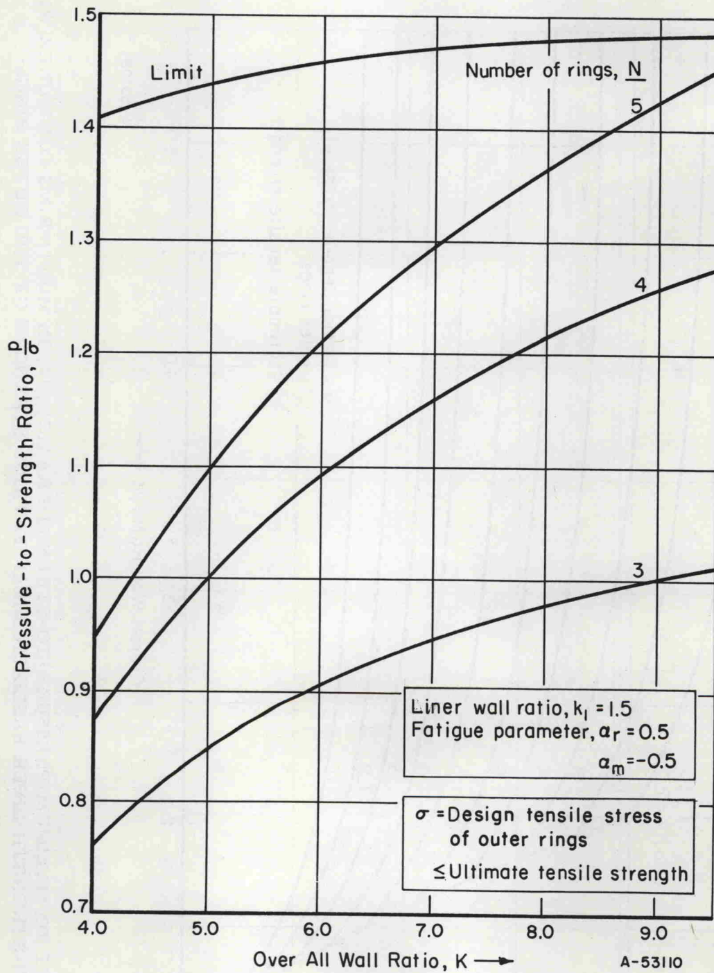
FIGURE 14. INFLUENCE OF NUMBER OF RINGS ON MAXIMUM PRESSURE-TO-STRENGTH RATIO, p/\sigma , IN MULTI-RING CONTAINER WITH HIGH-STRENGTH LINER
